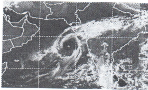
IR Satellite imagery at 1100 PST on 27 October 2019
